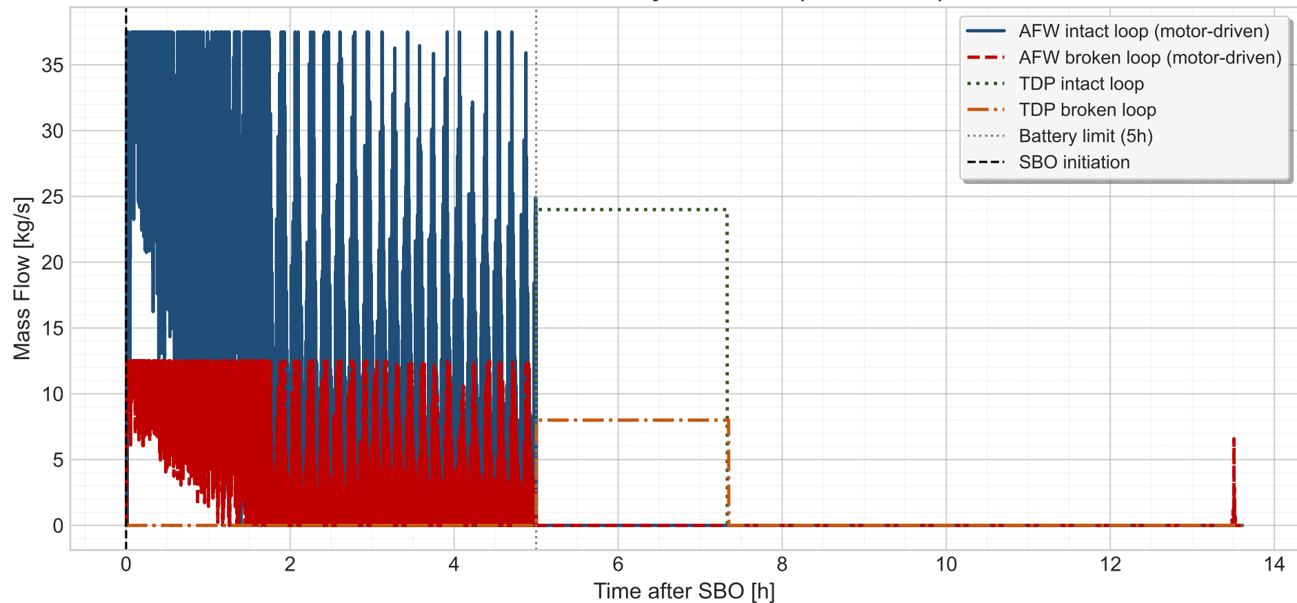
Base Case - Auxiliary Feedwater (AFW & TDP)
